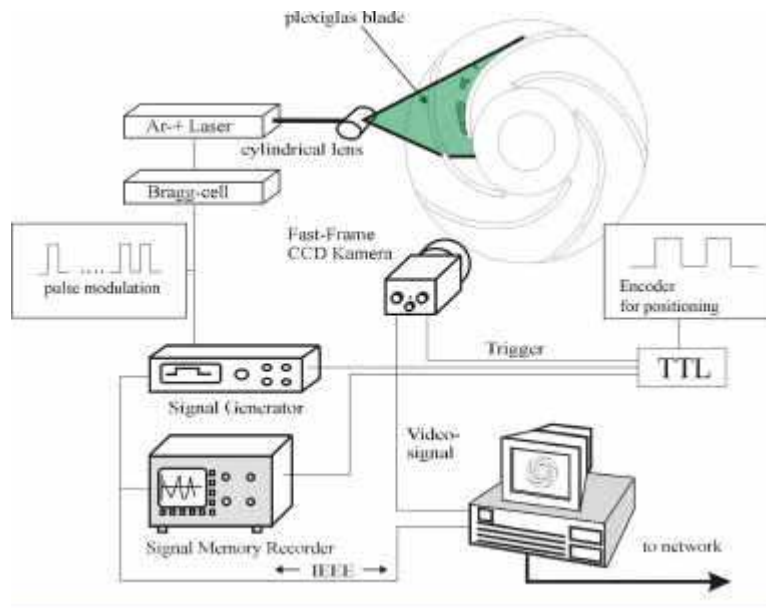
Figure 2. Visualisation set-up
