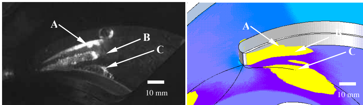
Figure 10. Vapour structures on suction side (experiment NPSH=8m, computation NPSH = 7m). Calculation: iso-density contour ( \rho \approx 0.95\rho_p ; void ratio >5%) drawn in yellow, shroud in blue, blade in grey
