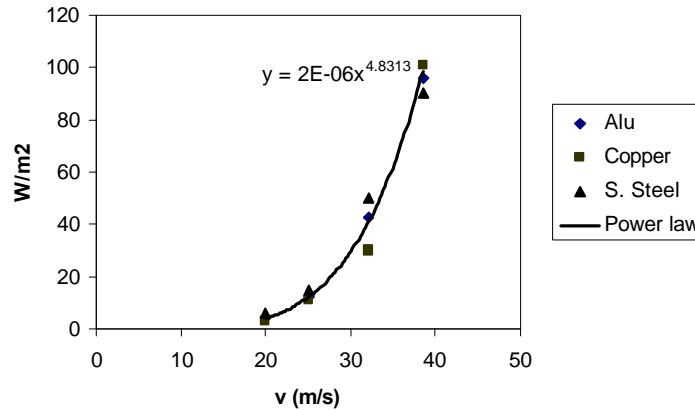
Figure 7: Pressure wave power density (measured by three different materials) as a function of the flow velocity.
