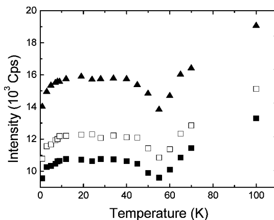
Fig. 7 Evolution of the background at low diffraction angles versus temperature for 2\theta values of 2.3, 2.4 and 2.5^\circ (from top to bottom).
