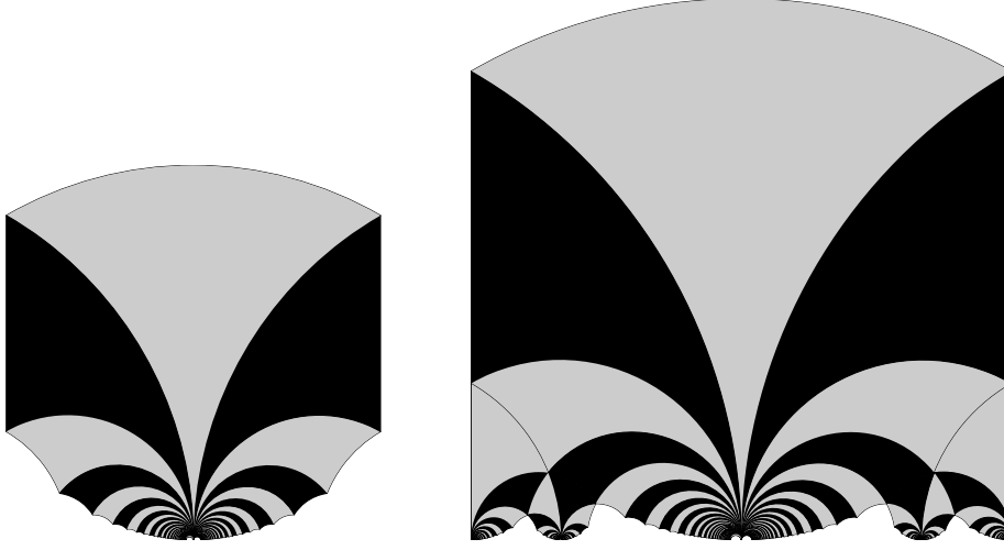
Figure 5: On the left, the “central” festoon \mathcal{F}_{(0,1)} . On the right, three festoons of the strip \mathcal{B} , relative to (0, 1), (1, 3), (-1, 3) and the two half-festoons at (-1, 2) and (1, 2) .
