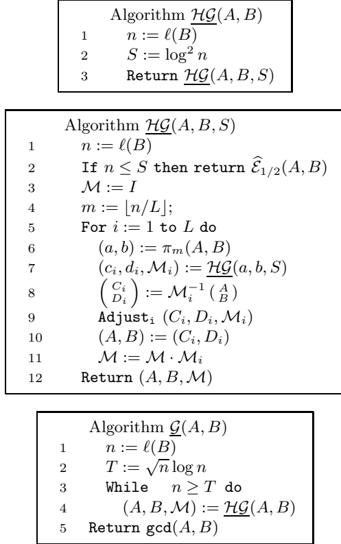
Figure 4: General structure of the algorithms \mathcal{H}\mathcal{G} and \mathcal{G} to be analyzed. The integer L \geq 2 defined as L := \max(2, \lceil 4/\sigma \rceil) depends, via the strip width \sigma , on the US property of the Euclidean Algorithm.
