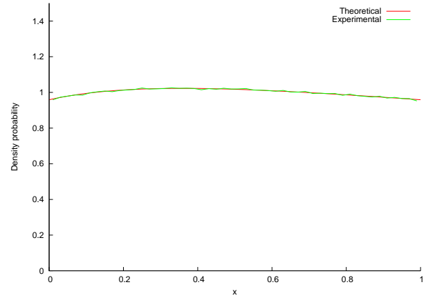
Figure 1: Density distribution of x_{\langle \delta \rangle} in the case \delta = 1/2 . This corresponds to the density distribution of the rational x_k := A_{k+1}/A_k obtained as soon as \ell(A_k) is smaller than (1/2)\ell(A_0) . The density distribution is plotted against its theoretical counterparts \psi(x) . Here we consider \Omega_n for n = 48 (48 bits), the interval [0, 1] is subdivided into equal subintervals of length 1/50 to estimate the density, and 3 537 944 rational are drawn from \Omega_n according to the initial density distribution \varphi by Monte Carlo simulation.
