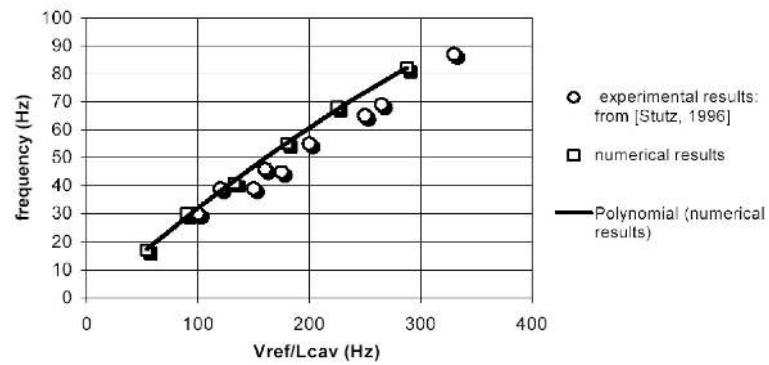
Figure 5: Experimental and numerical oscillation frequency.
