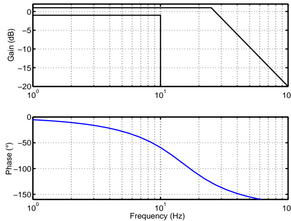
Figure 3: Bode template. Top - Gain (dB) versus frequency (Hz). Bottom . Phase (deg) versus frequency (Hz).
