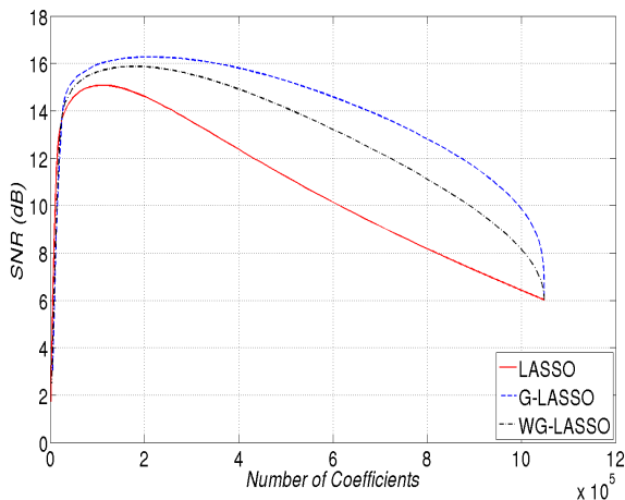
Fig. 8 Multichannel denoising of the train signal. SNR as a function of the number of retained coefficients; full curve: LASSO; dashed curve: G-LASSO; dashed-dotted curve: WG-LASSO.
