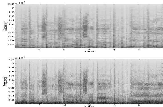
Fig. 10 MDCT coefficients of the signal. Top: in \mathbf{U} , bottom: in \mathbf{V} .
