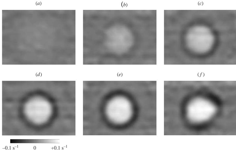
FIGURE 3. Time sequence of the vertical vorticity field from PIV measurements in a horizontal plane 2 cm above the disk showing the generation of cyclonic vorticity by stretching of background vorticity and the formation of an anticyclonic ring above the growing density front for \Delta t = 50.0 . Experimental parameters are: f = 0.26 \text{ s}^{-1} , N = 1.4 \text{ s}^{-1} , \omega_d = 0.24 \text{ s}^{-1} , R = 12 \text{ cm} , and (a) t = 0 , (b) 50, (c) 100, (d) 150, (e) 200 and (f) 250 s.
