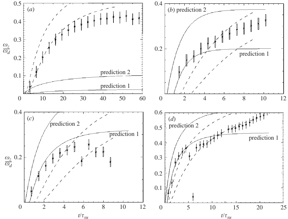
FIGURE 8. Evolution of the vertical vorticity \omega_z 2 cm above the centre of the rotating disk for experiments (a) c , (b) h , (c) j and (d) F (see tables 1 and 2 for experimental parameters). Dashed lines: the diffusive model for heights 1.75 cm and 2.25 cm; solid line labelled prediction 1 : the stretching model for L = 0.5 , height 2.25 cm and a delay for the initial time ( \sim 4\pi/(f + wd) ) in order to reproduce the formation of the Ekman layer; solid line labelled prediction 2 : the stretching model for L = 1.5 , height 1.75 cm, without delay. *, experimental values based upon PIV measurements.
