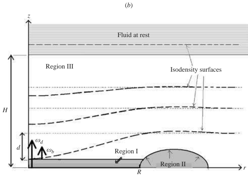
FIGURE 5. (a) Side-view dye visualization of the spin-up flow in its final state, illustrating the deviation of the density field. The black streaks represent the fluoresceine dye planes illuminated by a vertical laser plane at t=48 min, whereas the white lines represent their initial position at t=0 (colours in the image are inverted). (b) Schematic of the flow for the stretching model, with region I the boundary layer, region II the density front generated by ejected fluid of region I, and region III, where fluid is spin-up by stretching and compression of background vorticity, extending to a limited height H because of the stratification. \omega_b and \omega_d are the vertical vorticity at the base of region I and of the rotating disk, respectively.
