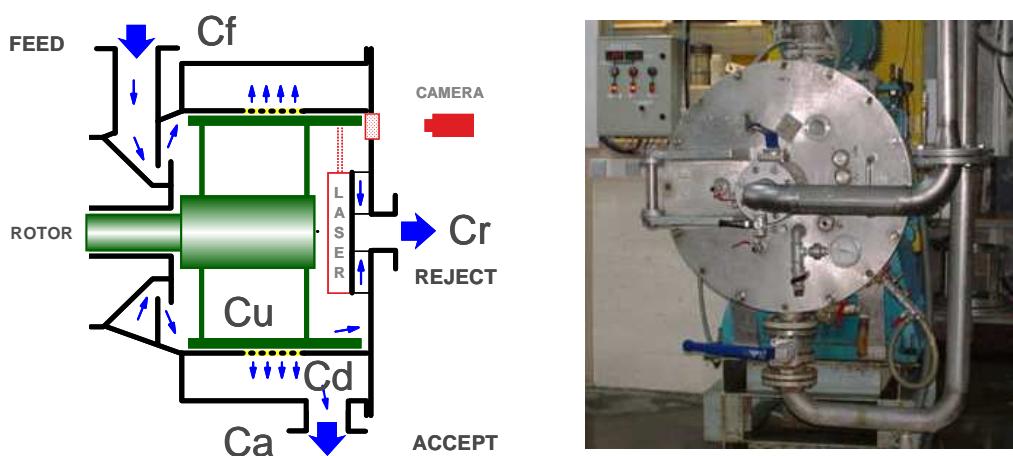
Figure 15: Experimental “slice screen” – 500 mm screen cylinder diameter
