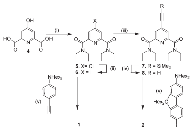
Scheme 1 (i) SOCl 2 , DMF (cat.), reflux, followed by HNEt 2 , CH 2 Cl 2 , reflux, 72%; (ii) HI (aq.), H 3 PO 3 (cat.), 80 °C, 3.5 h, 62%; (iii) TMS-CCH, PdCl 2 (PPh 3 ) 2 , CuI, THF-NEt 3 , 40 °C, 91% (iv) K 2 CO 3 , MeOH-CH 2 Cl 2 , 94%; (v) PdCl 2 (PPh 3 ) 2 , CuI, THF-NEt 3 , 40 °C, 89% ( 1 ), 53% ( 2 ).
