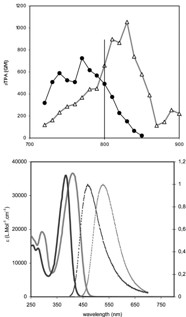
Fig. 2 Absorption and normalized emission (dashed lines) (down) and two-photon excitation (up) spectra of 1 (black) and 2 (gray) in chloroform.
