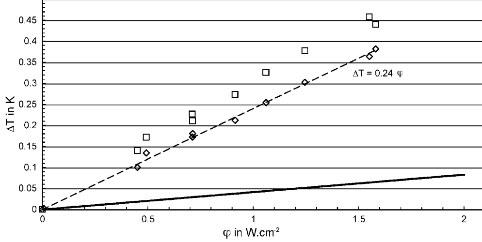
Fig. 9. Temperature measurement error as a function of applied heat flux. □ T_{\text{iso}} - T_{\text{cold}} , ◇ T_{\text{hot}} - T_{\text{iso}} — Pure conduction in brass over 0.5 mm.
