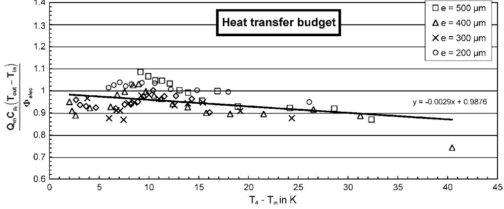
Fig. 4. Heat transfer budget as a function of temperature difference T_4 - T_{in} for \Phi_{elec} = 180 W.
