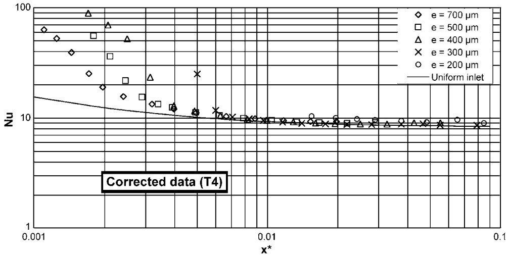
Fig. 11. Evolution of Nu(x^*) as a function of the channel spacing e at the abscissa corresponding to T4 ( \Phi_{\text{elec}} = 180 \text{ W} )—corrected results.
