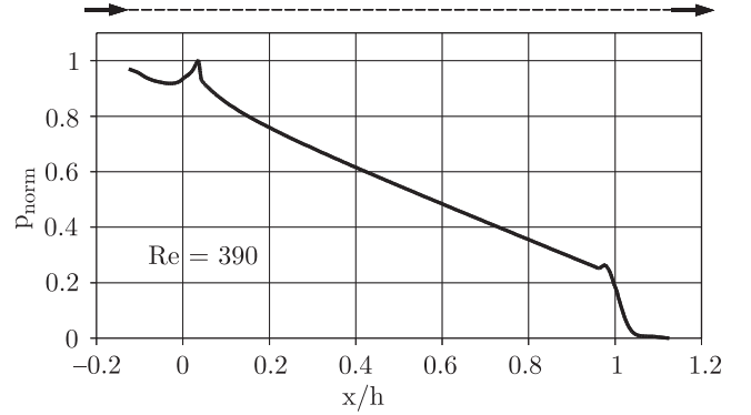
Fig. 17. Pressure variation along the centreline of the system
