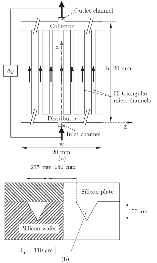
Fig. 3. The geometry of microchannels system; entire view of the network (a); cross-sectional view of silicon wafer (b)
