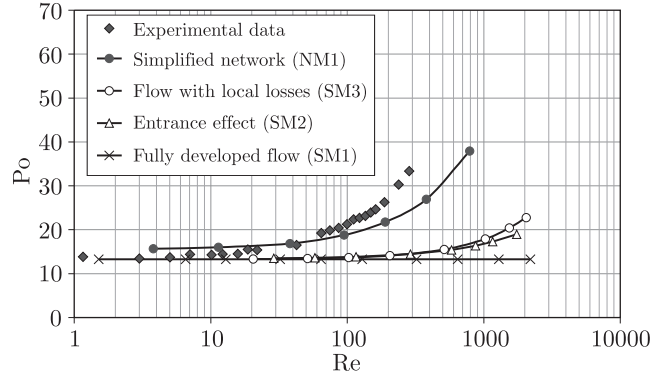
Fig. 10. Contribution of the mixing to the flow resistance of the microchannels system
