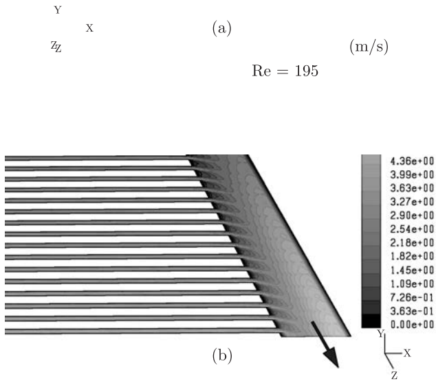
Fig. 12. Velocity vector magnitude distribution; inside the distributor (a); inside the collector illustrating mixing losses (b)
