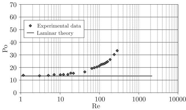
Fig. 4. Pressure losses in a system of microchannels – experiment versus fully developed flow (after Ref. 9)
