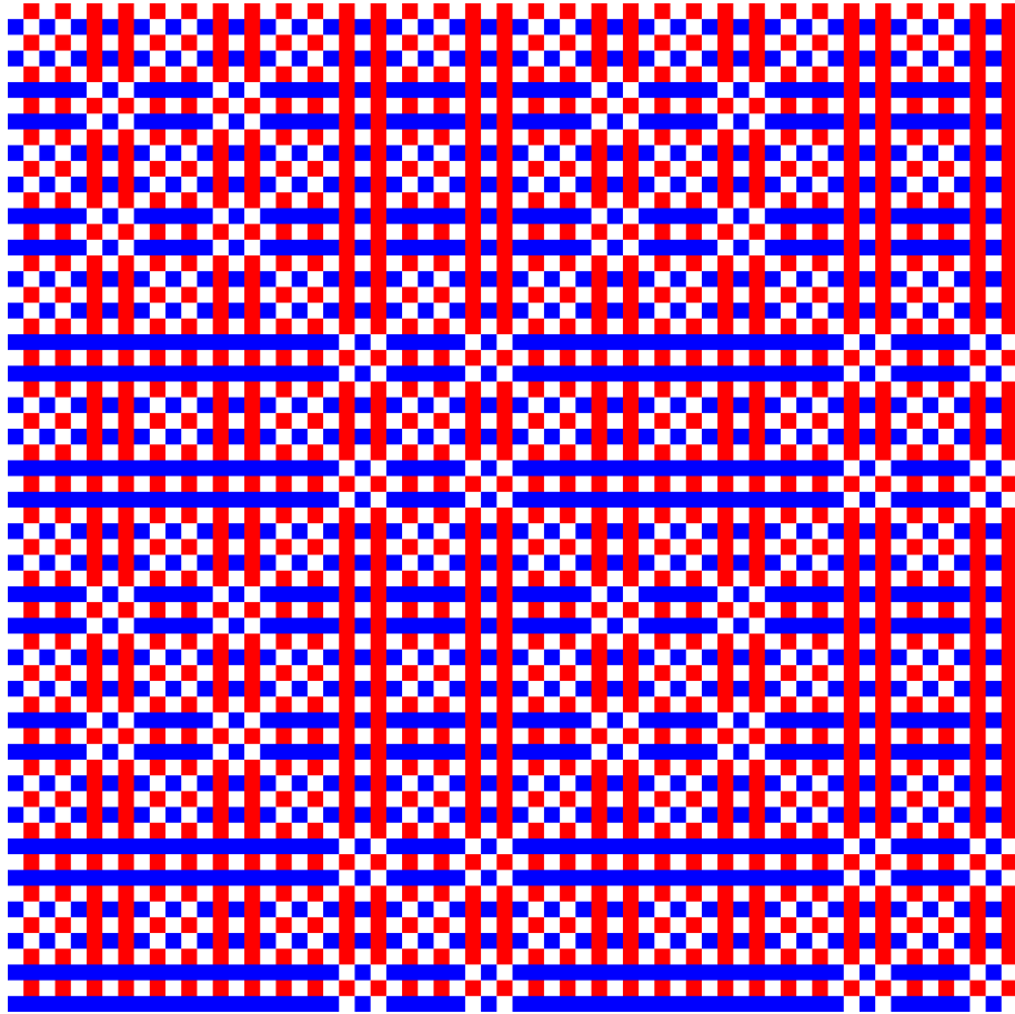
Fig. 9: Detail of \mathcal{A}_\epsilon
