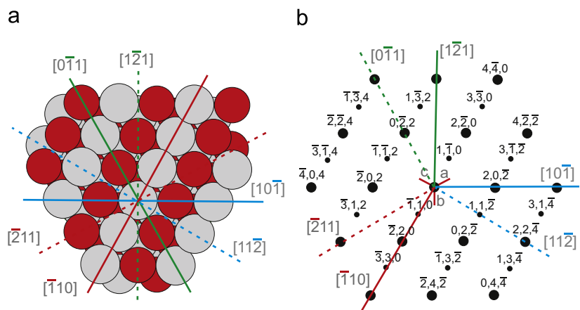
Fig. 2. (a) Schematic view of the (111) plane of the one variant of the L1_0 phase formed with the tetragonal axis along [001] ; and (b) the reciprocal plane corresponding to the [111] zone axis.
