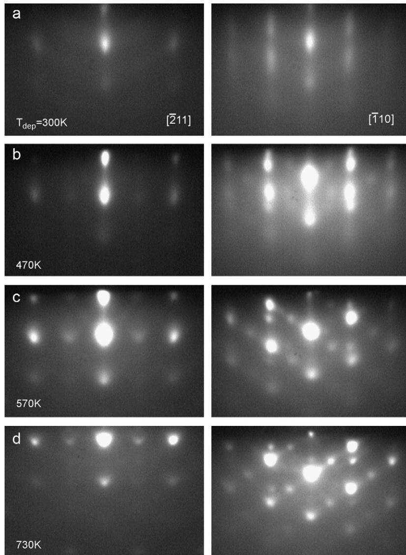
Fig. 1. RHEED patterns taken after the deposition of 3-nm-thick CoPt alloy on \text{WSe}_2(0001) at various temperatures: (a) 300 K, (b) 470 K, (c) 570 K, and (d) 730 K.
