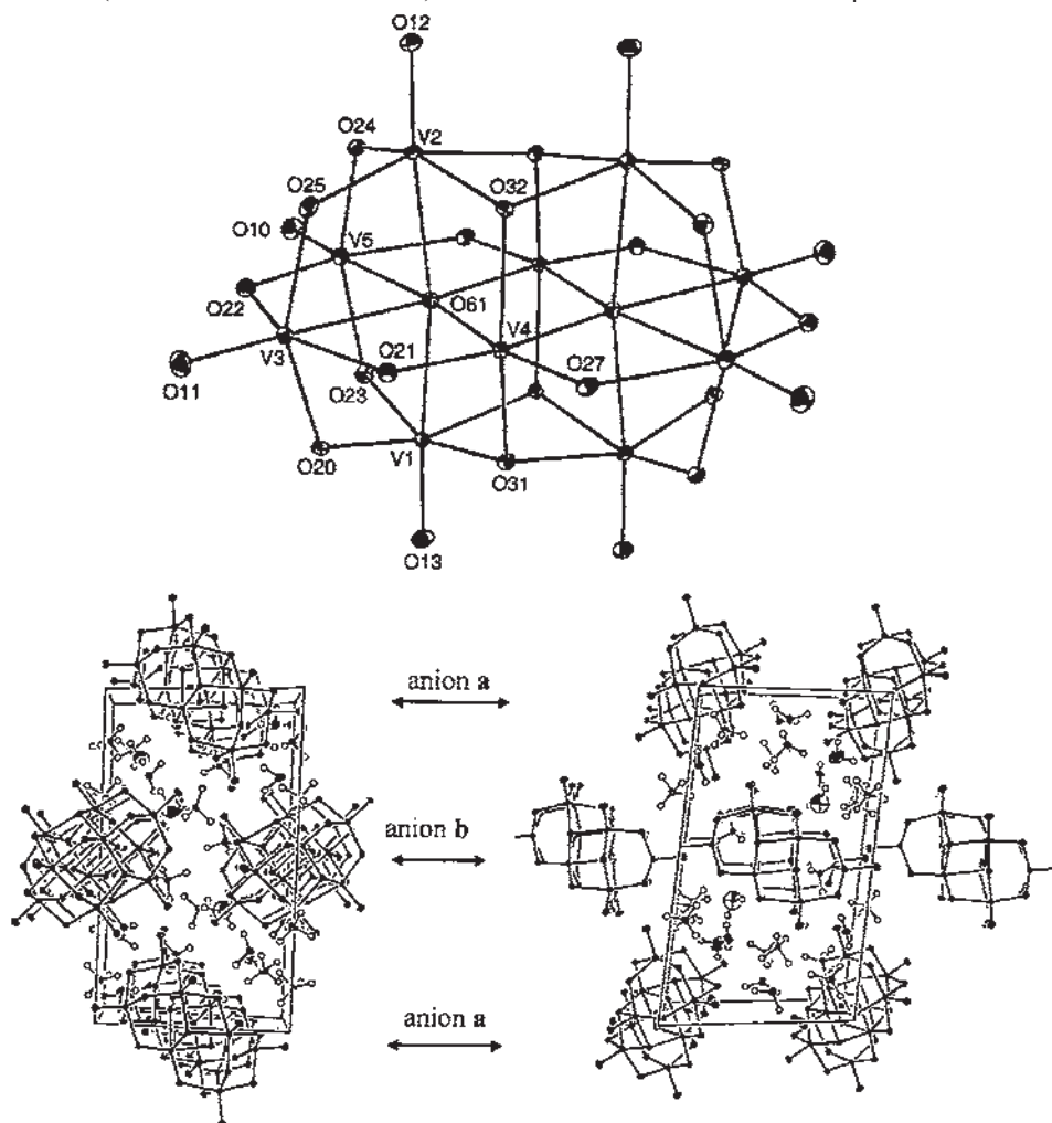
Fig. 1. ORTEP view of the decavanadate anion with the atomic labelling scheme (top) and crystal lattice packing (bottom) of ammonium decavanadate hexahydrate.
