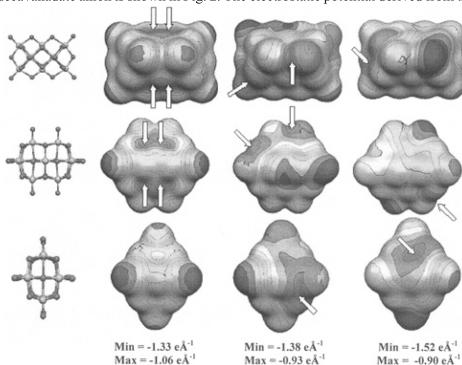
Fig. 2. Three views of the electrostatic potential on the van der Waals surface of the decavanadate polyanion: from Mulliken population analysis (second column, from 22 ); from decavanadate a experimental charges (third column); from decavanadate b experimental charges (fourth column). The arrows indicate the minima of the electrostatic potential and the maximum regions are in black.
