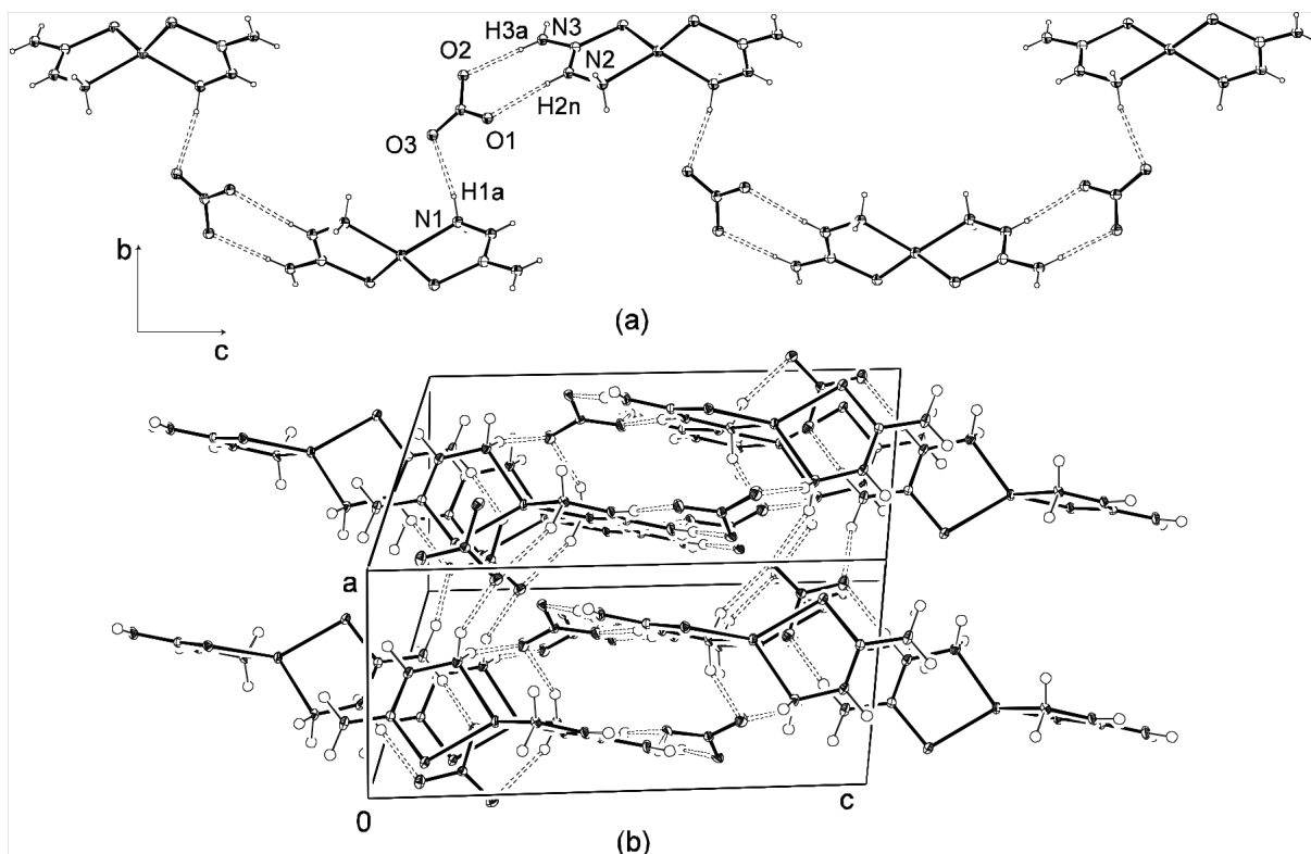
Figure 3. (a) One dimensional chain formed by the strongest hydrogen bonds; (b) segment of the crystal packing of [\text{Zn}(\text{TSC})_2](\text{NO}_3)_2 .
