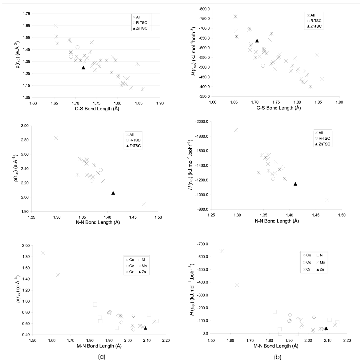
Figure 5. \rho(r_c) vs bond length (a) and H(r_c) vs bond length (b) for C-S, N-N and M-N bonds. 36-38 (R-TSC is for other TSC based compounds 20,21 ).
