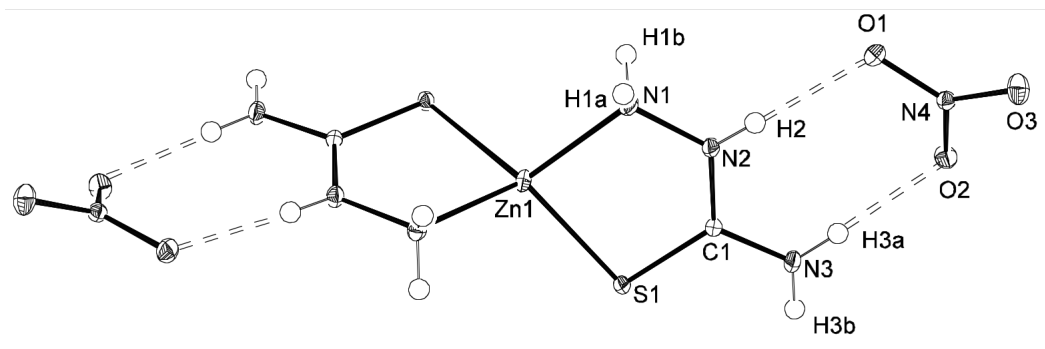
Figure 2. Crystal structure of [\text{Zn}(\text{TSC})_2](\text{NO}_3)_2 .
