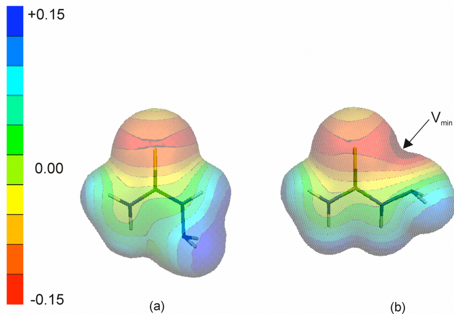
Figure 9. Theoretically determined EP ( e \cdot \text{\AA}^{-1} ) generated on the three-dimensional isodensity surface ( 0.007 e \cdot \text{\AA}^{-3} ) of the TSC ligand in: (a) trans ; (b) cis -configuration.
