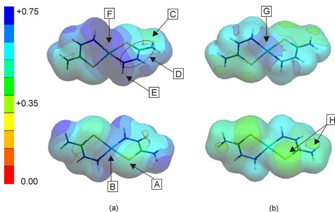
Figure 8. EP ( e \cdot \text{\AA}^{-1} ) generated on the cationic three-dimensional isodensity surface ( 0.007 e \cdot \text{\AA}^{-3} ): (a) experimental; (b) theoretical (DFT).
