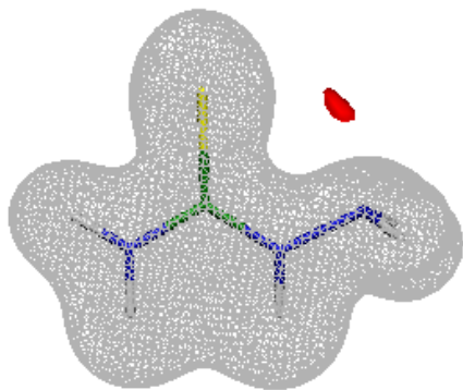
Figure 10. Three-dimensional isopotential surfaces of the coordinated form ( cis ) of the TSC ligand; Grey and red correspond to V_{\max} = +0.18 and V_{\min} = -0.18 \text{ e} \cdot \text{Å}^{-1} , respectively.
