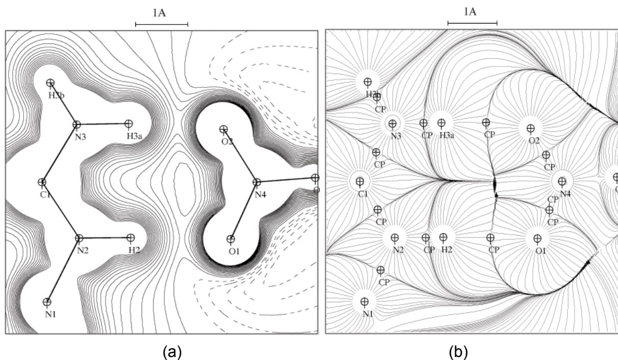
Figure 12. (a) Electrostatic potential in the TSC-NO 3 double hydrogen bonds plane. Contour intervals 0.05 eÅ -1 ; negative contours are dashed, zero contour omitted. (b) Electric field lines in the same plane. Critical points are indicated as “CP”.
