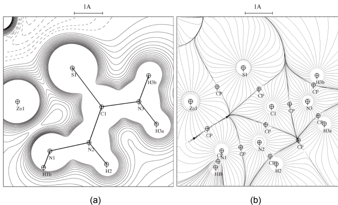
Figure 11. (a) Electrostatic potential in the Zn-TSC ligand plane. Contour intervals 0.05 \text{ e}\text{\AA}^{-1} ; negative contours are dashed, zero contour omitted. (b) Electric field lines in the same plane. Critical points are indicated as “CP”.
