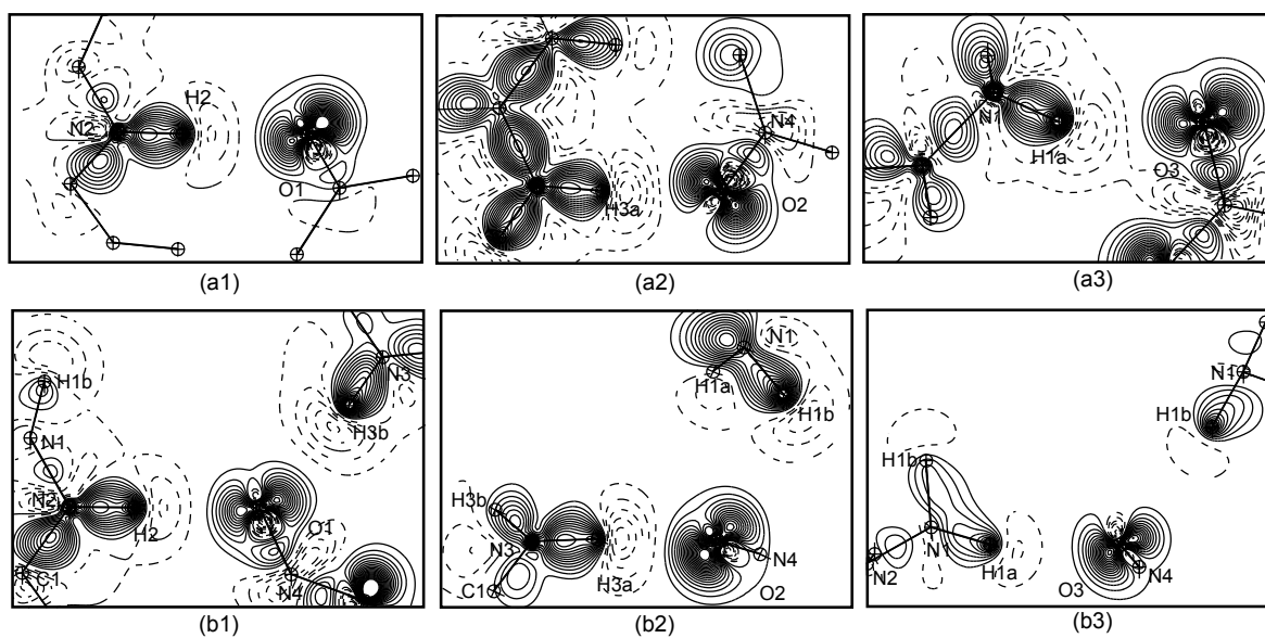
Figure 7. Hydrogen bonds static electron deformation density maps: (a) The maps are plotted in the plane containing the strongest hydrogen bond connected respectively to O1, O2 and O3; (b) The maps are plotted in the plane defined by the oxygen atom and the pair of hydrogen atoms which form two strongest hydrogen bonds. The contour interval is 0.05 \text{ e} \cdot \text{\AA}^{-3}
