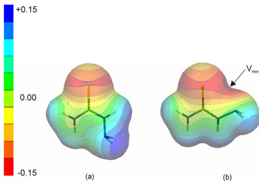
Figure 9. Theoretically determined EP ( \text{e} \cdot \text{\AA}^{-1} ) generated on the three-dimensional isodensity surface ( 0.007 \text{ e} \cdot \text{\AA}^{-3} ) of the TSC ligand in: (a) trans ; (b) cis -configuration.
