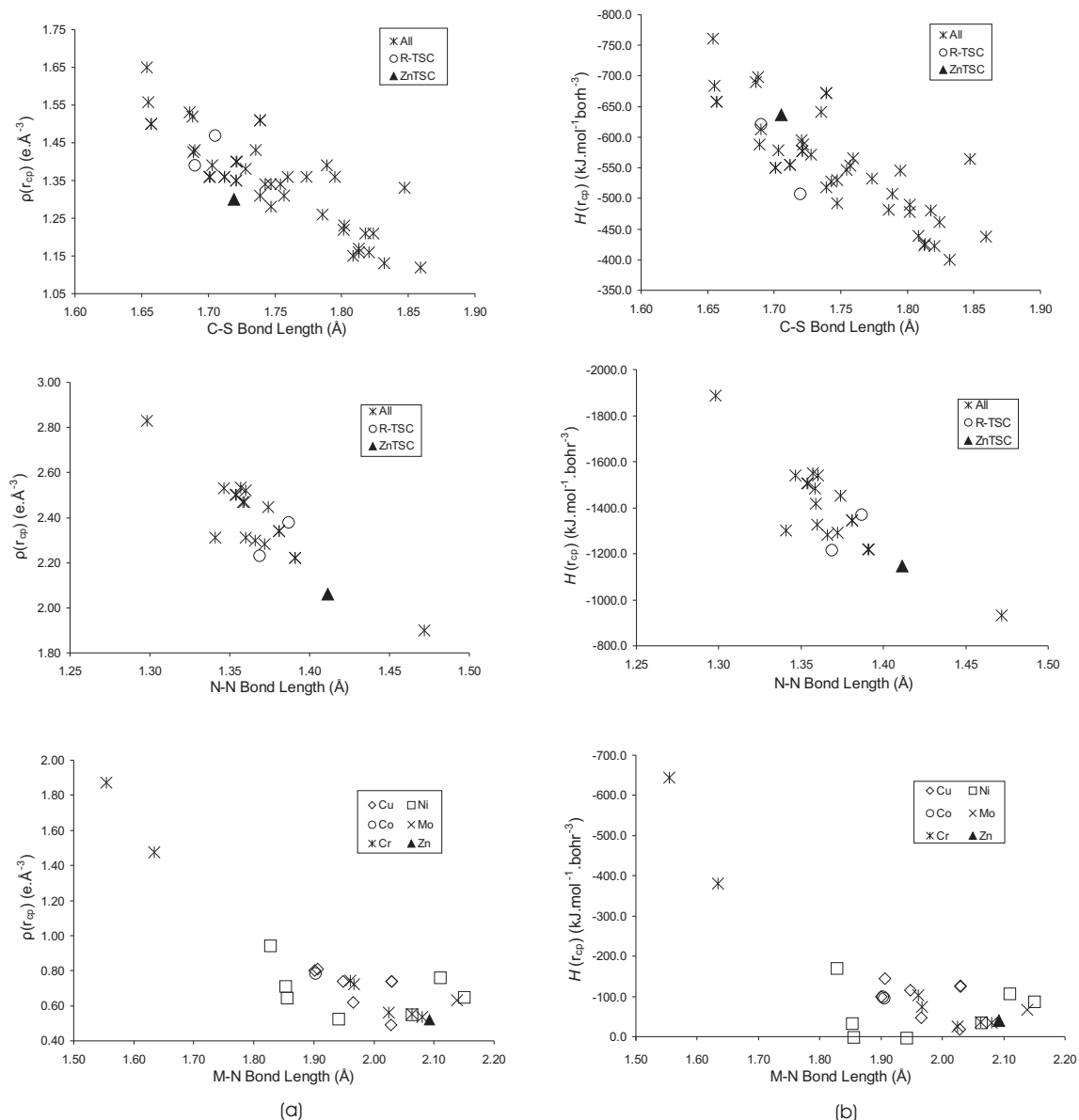
Figure 5. \rho(r_c) vs bond length (a) and H(r_c) vs bond length (b) for C-S, N-N and M-N bonds. 36-38 (R-TSC is for other TSC based compounds 20,21 ).
