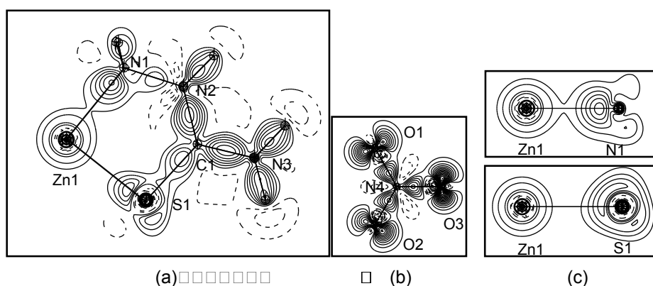
Figure 4. Static electron deformation density maps (a) Zn1-C1-N1 plane; (b) N4-O3-O1 plane; (c) in the plane orthogonal to the chelate ring. Contours are as in Figure 1.
