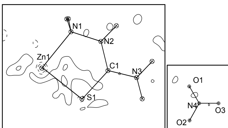
Figure 1. Residual electron density maps: (a) Zn1-C1-N1 plane; (b) N4-O3-O1 plane. The contour interval is 0.1 \text{ e} \cdot \text{\AA}^{-3} ; negative contours are dashed, zero contour omitted.
