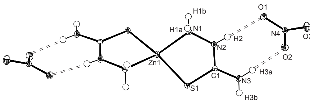
Figure 2. Crystal structure of [\text{Zn}(\text{TSC})_2](\text{NO}_3)_2 .
