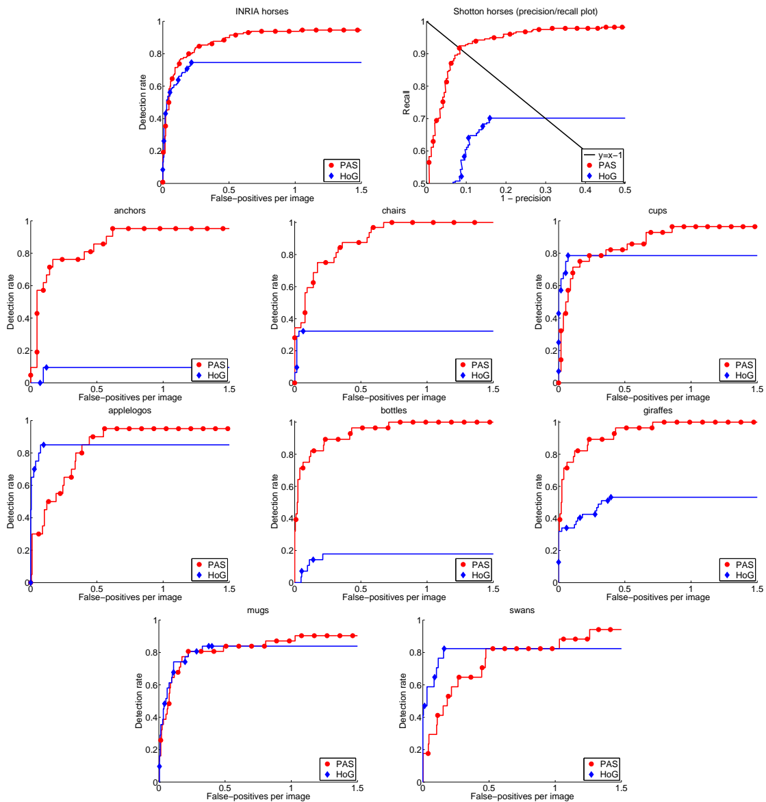
Fig. 13. Comparison between our PAS-based detector and Dalal and Triggs [4] HoG-based one.
