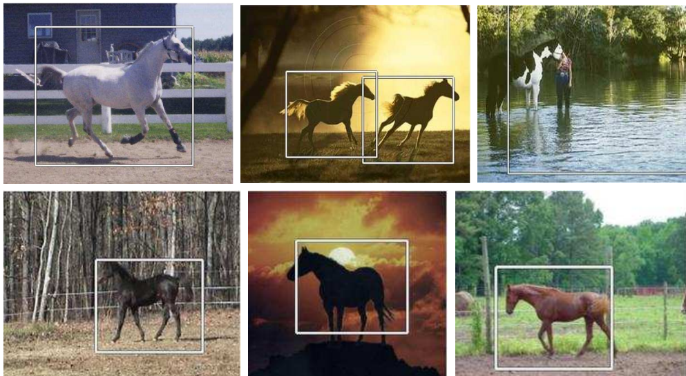
Fig. 8. Top row: detections at 0.4 FPPI for the INRIA horses dataset. The rightmost image shows a missed detection and a false-positive. Bottom: detections at the equal-error rate for the Shotton horses dataset.
