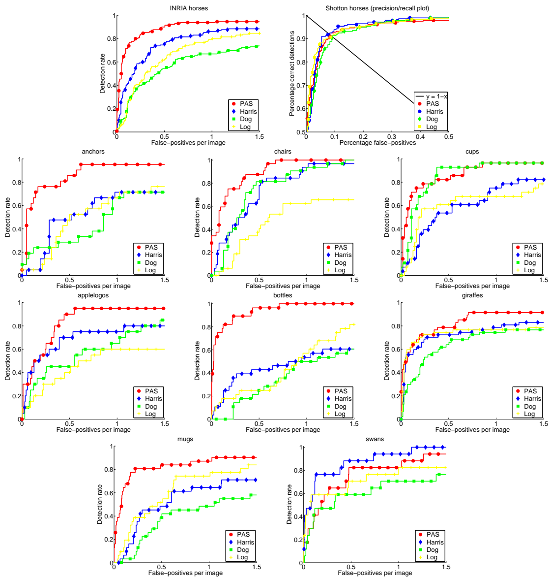
Fig. 12. Performance of interest points compared to PAS.
