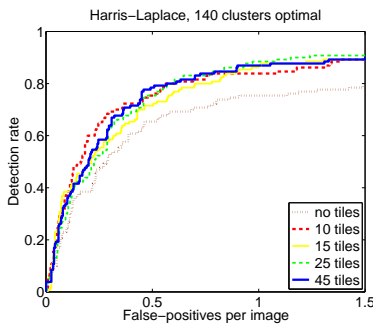
Fig. 11. Optimizing T with the number of clusters fixed at 140 (which is the optimum in the tested range 100–300).
