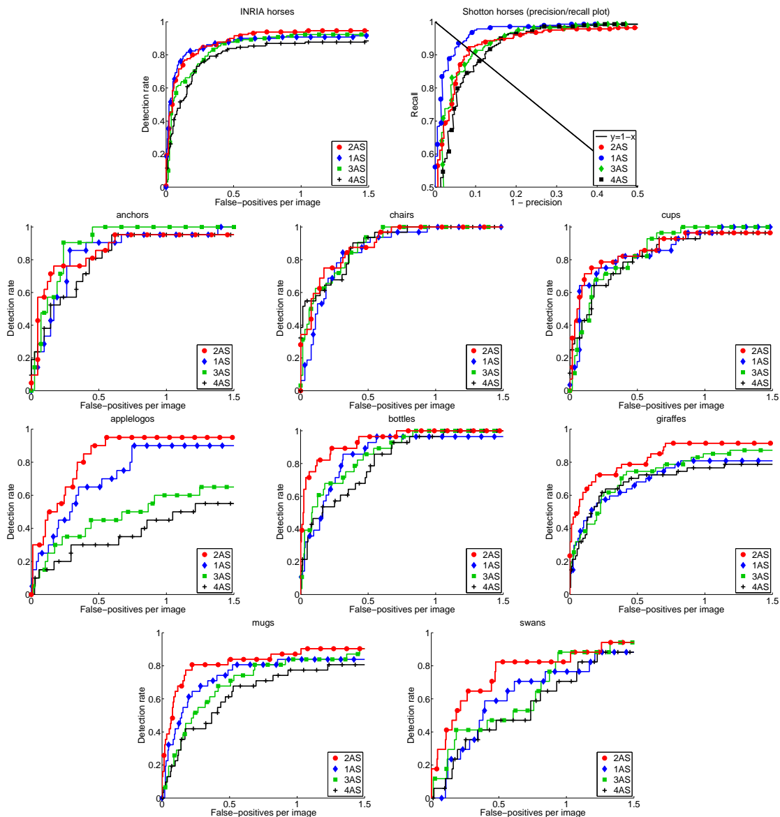
Fig. 9. Performance of kAS , for varying degrees of complexity k . Top row: the two horses datasets: INRIA horses and Shotton horses. Second row: the three classes from Caltech 101. Third row: the five ETHZ shape classes. All performance comparison figures in the paper follow this layout.
