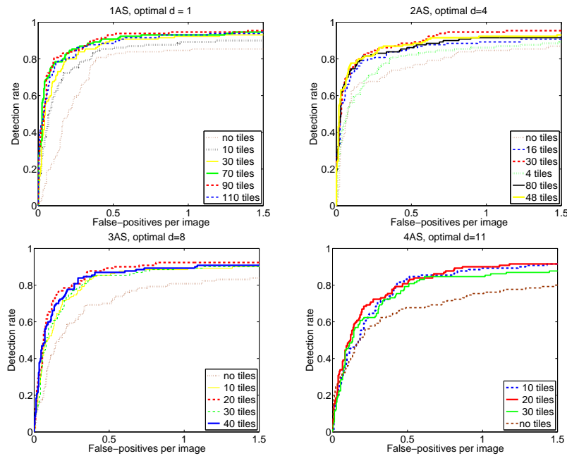
Fig. 7. Impact of window tiling resolution T at the optimal clustering threshold d . The optimum is T = 90 for 1AS, T = 30 for 2AS, and T = 20 for 3AS and 4AS.
