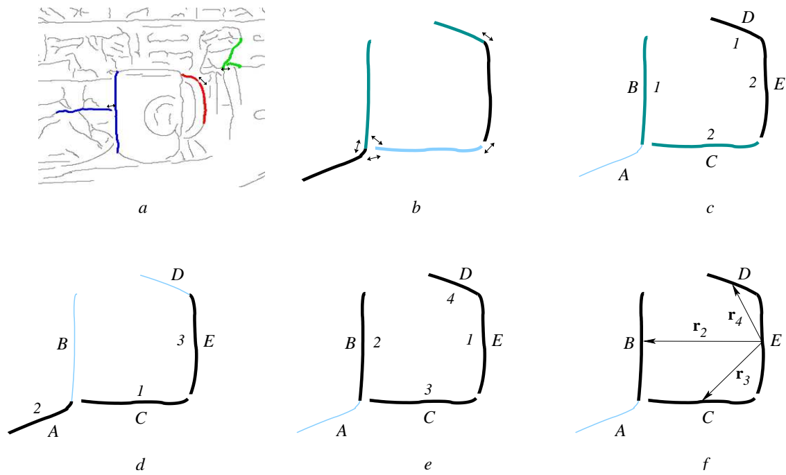
Fig. 1. a) An example image, with three 2AS and the underlying CSN connections (arrows). Notice how one 2AS lies entirely on the boundary of a mug. b) Three edgel-chains, with five segments and their inter-connections (arrows) in the network. c) Two detected 2AS ( B, C ) and ( D, E ). The order of each segment in the descriptor is marked next to it (see section III-B). Notice that ( A, B ), ( A, C ), ( C, E ) are also detected, though not displayed because they overlap with ( B, C ) and ( D, E ). d) 3AS ( C, A, E ). e) 4AS ( E, B, C, D ). f) r_i vectors involved in the description of the 4AS in d ).
