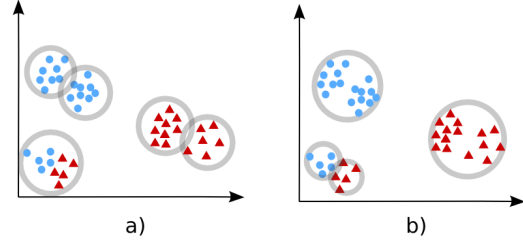
Fig. 2: Clustering algorithms: a) Unsupervised clustering algorithm b) Supervised clustering algorithm.
