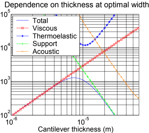
Figure 3: Quality factors (log scale) at the optimal width ( 37 \mu\text{m} ) for a 100 \mu\text{m} long microcantilever as a function of the thickness (log scale)
