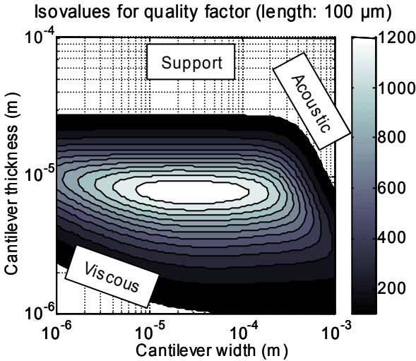
Figure 2: Total quality factor and dominant losses for a 100 \mu\text{m} long microcantilever as a function of the microcantilever width and thickness
