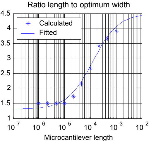
Figure 5: Ratio length to optimum width for different microcantilever lengths (calculated values and fitted model)
