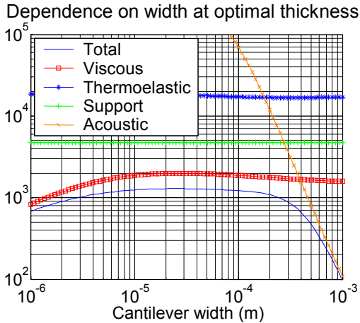
Figure 4: Quality factors (log scale) at the optimal thickness ( 7.7 \mu\text{m} ) for a 100 \mu\text{m} long microcantilever as a function of the width (log scale)
