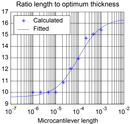
Figure 6: Ratio length to optimum thickness for different microcantilever lengths (calculated values and fitted model)
