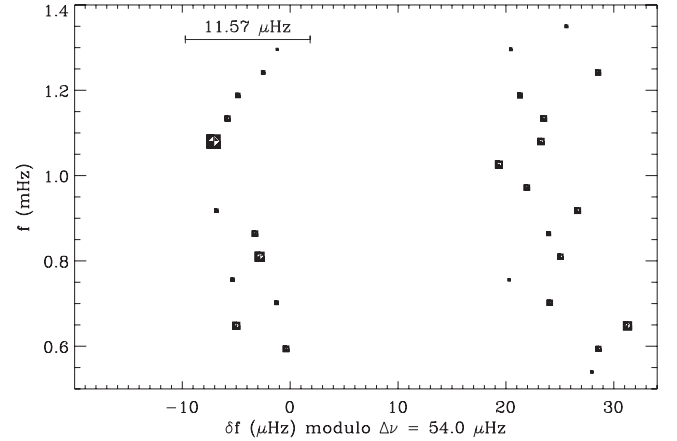
Fig. 6. Échelle diagram, selecting only the major peaks detected in Fig. 4, and excluding the peaks present in the neighboring aliases of the ridge around -6 \mu\text{Hz} (modulo 54 \mu\text{Hz} ), identified to \ell = 1 modes. The other ridge includes \ell = 0 and, maybe, 2 modes. The highest confidence levels are reached for the peaks identified above 1 mHz, which exhibit large spacings about 55 \mu\text{Hz} .
