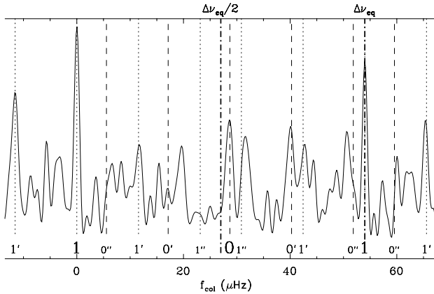
Fig. 5. Rescaled collapsogram of the échelle diagram of Fig. 4, based on the \ell = 1 ridge and rescaled on a fixed value of the large frequency spacing. The signature of \ell = 0 mode is clearly identified, slightly greater than half the large spacing (dot-dashed line), but there is no clear detection of \ell = 2 modes. Most of the peaks are related to the \ell = 0 (dashed lines) and \ell = 1 (dotted lines) modes, or to their aliases at \pm 11.6 \mu\text{Hz} (') or \pm 23.2 \mu\text{Hz} (''). The alias at -23.2 \mu\text{Hz} of the \ell = 1 ridge appears to be boosted in the vicinity of the \ell = 0 ridge.
