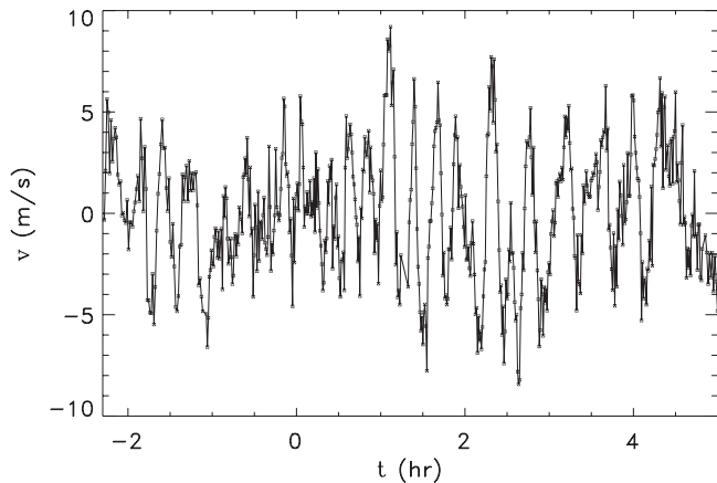
Fig. 2. Zoom of the radial velocity curve (1st night). Oscillations with a period about 17 min are clearly visible.
