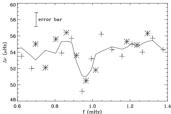
Fig. 7. Large spacing as a function of frequency, for the degrees 0 (+), 1 (*) (after disentangling of \ell=0 and 2 modes), and global fit (solid line) corresponding to the boxcar average smoothed over 3 consecutive values. Error bars, estimated according to Libbrecht (1992), are about 1.6 \mu\text{Hz} . As in Martić et al. (2004), a lower value of the large spacing is observed in the frequency range [0.9, 1.0 mHz]. Outside this range, the large spacing increases with frequency.
