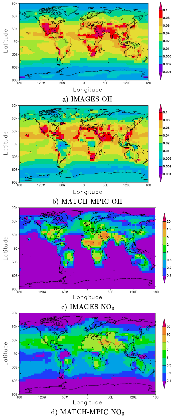
Fig. 7. Annually-averaged OH and NO 3 mixing ratios (ppt) at the surface in IMAGES (a, c) (EXP1) and MATCH-MPIC (b, d) (EXP5).
