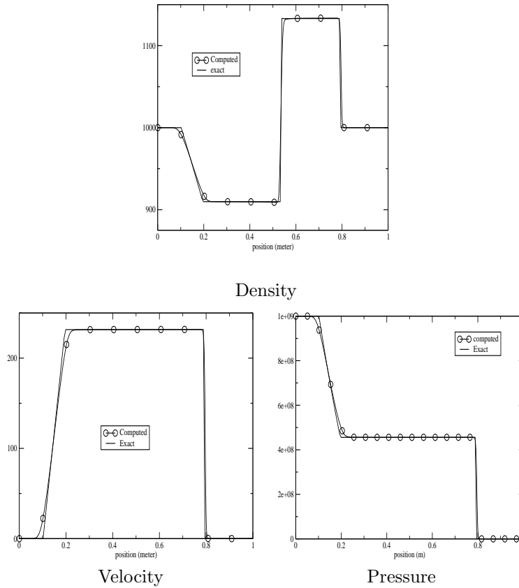
FIG. 3. Single fluid problem: approximated solution (circles) and exact solution (solid).
