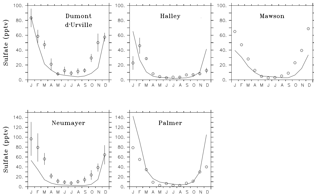
Figure 6. Seasonal variations of nss sulfate (pptv) near the ground at the Antarctic stations Dumont-d'Urville ( 140^{\circ}1'E , 66^{\circ}40'S ), Halley ( 26^{\circ}19'W , 75^{\circ}35'S ), Neumayer ( 8^{\circ}15'W , 70^{\circ}39'S ) [Minikin et al. , 1998], Palmer ( 64^{\circ}03'W , 64^{\circ}46'S ), and Mawson ( 62^{\circ}30'E , 67^{\circ}36'S ). Open circles represent monthly mean observed concentrations [Minikin et al. , 1998; Savoie et al. , 1993]. Standard deviations of monthly values (representing year-to-year variability) are plotted as vertical lines. Model results are shown as solid lines.
