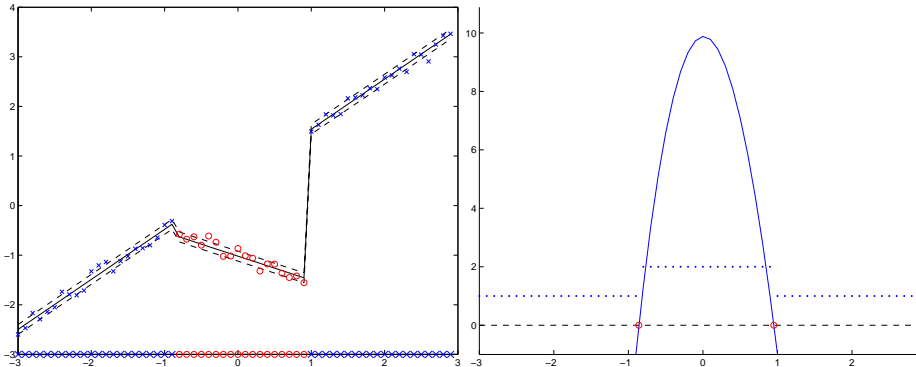
Fig. 2. Nonlinear boundary between 2 modes. Left: Hybrid model (—) with its insensitivity tube (- -) approximating the data points represented by 'x' for \hat{\lambda}_i = 1 and 'o' for \hat{\lambda}_i = 2 . The estimated mode \hat{\lambda}_i also appears on the x -axis as 'x' for mode 1 and 'o' for mode 2 to highlight the partition of the input space \mathcal{X} . Right: Class labels \hat{\lambda}_i (.) for each data point x_i used to learn the nonlinear boundary \mathcal{S} (o), defined as the zeros of h(x) (—).
