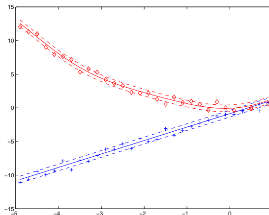
Fig. 1. One-dimensional example of the simultaneous estimation of two functions on noisy data. Points associated to the linear and RBF models are respectively represented by crosses (+) and diamonds (◇).
