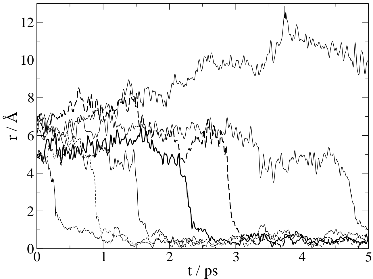
FIG. 6: Evolution of the electron-silver cation distance versus simulation time for seven different initial configurations of systems with 300 and 800 water molecules.
