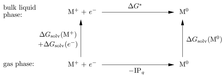
FIG. 5: Thermodynamic cycle for the reduction of a cation in bulk liquid phase.
