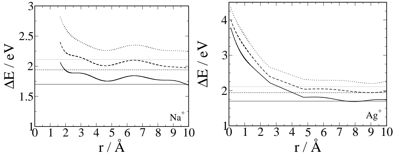
FIG. 4: Evolution of the energy difference between three first excited states and the ground state as a function of the electron-cation distance for sodium (left panel) and silver (right panel), with 800 water molecules. Full lines: (E_{p1} - E_0) , dashed line: (E_{p2} - E_0) and dotted line: (E_{p3} - E_0) . The horizontal lines correspond to the energies values obtained for the hydrated electron.
