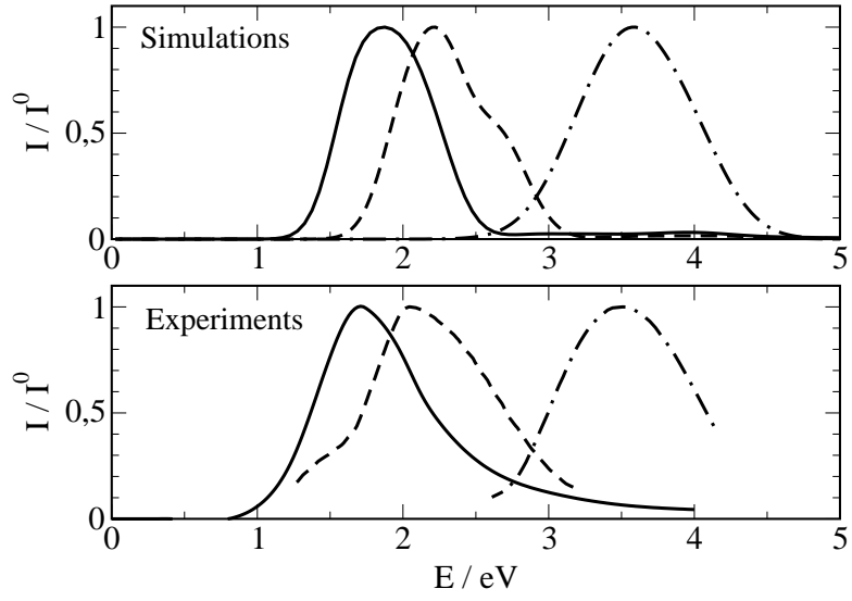
FIG. 1: Absorption spectra of an hydrated electron (solid line), in presence of a sodium cation (dashed line) and in presence of a silver cation (dashed-dotted line). Simulation results (top panel) and experimental data (lower panel).
