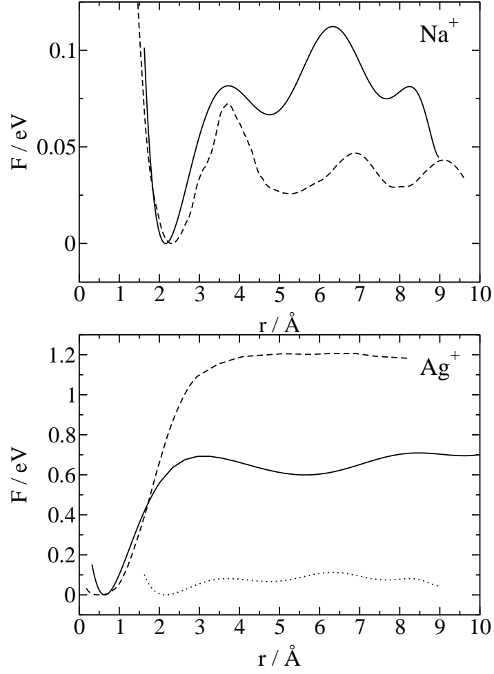
FIG. 2: Free energy profiles as a function of electron-cation distance obtained for sodium (left panel) and silver (right panel) simulations. In each case, the solid line is obtained with 800 water molecules, and the dashed line with 300 water molecules. The sodium curve for 800 water molecules is also plotted on the right panel (dotted line).
