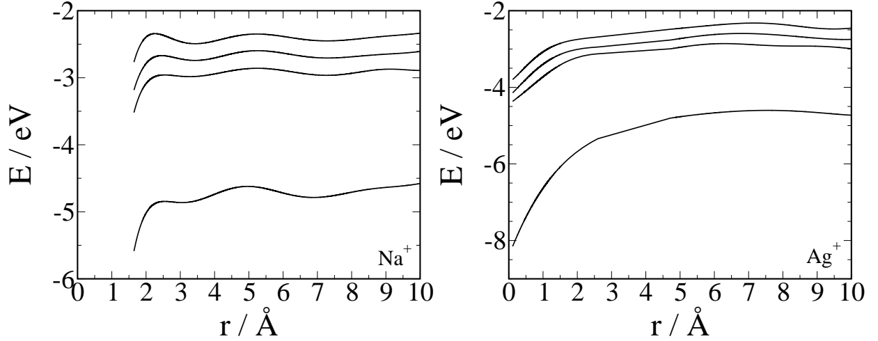
FIG. 3: Evolution of the energies of the ground state and the three first excited states as a function of the electron-cation distance sodium (left panel) and silver (right panel). The plotted values correspond to an average along constraint molecular dynamics runs for a box with 800 water molecules.
