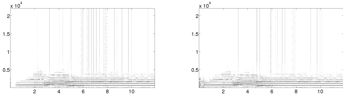
Fig. 4. Time-frequency representation of the Gabor coefficients for the denoised version. Left: \ell_1 estimate. Right: \ell_{1,2} estimate.
