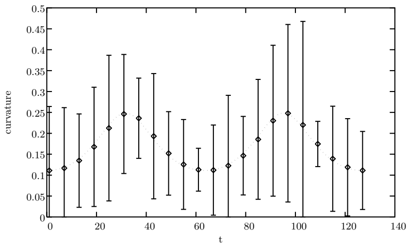
Figure 8. Experimental data ( \blacklozenge ) together with their uncertainty intervals and graph of the function \kappa(t) (see Eq. (23)).
