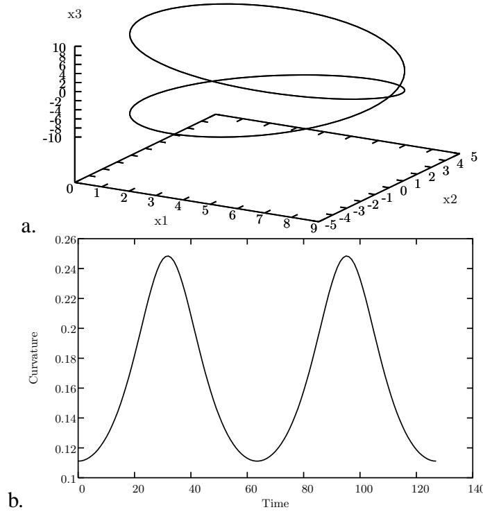
Figure 5. a. 3-dimensional representation of the Clelia curve. b. Graph of the function \kappa(t) given by equation (23).
