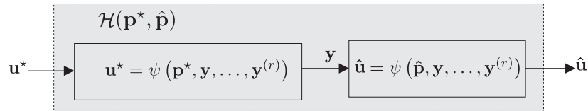
Figure 2. Système \mathcal{H}(\mathbf{p}^*, \hat{\mathbf{p}}) .
