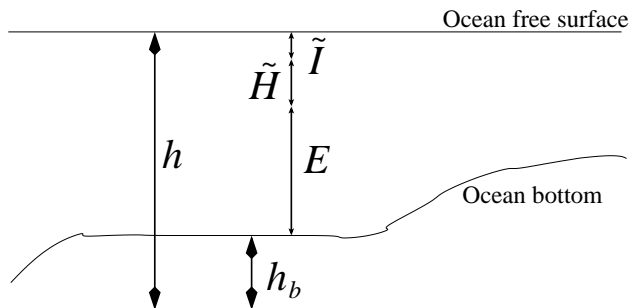
Figure 1: Fields h , h_b , E , \tilde{\mathcal{H}} and \tilde{\mathcal{I}}
