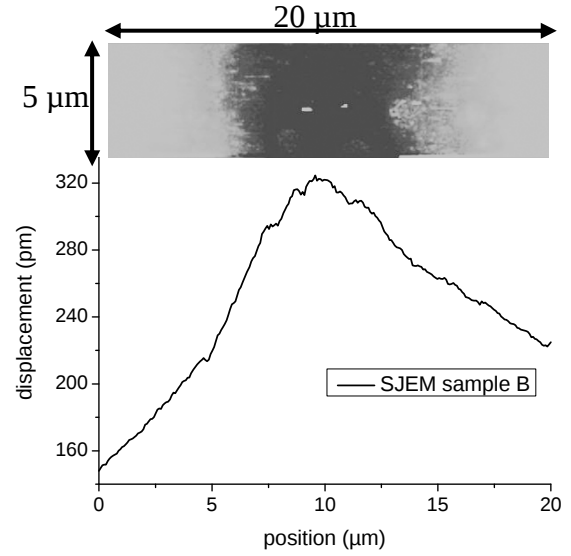
Fig. 5. SJEM expansion amplitude image and section (sample B).
