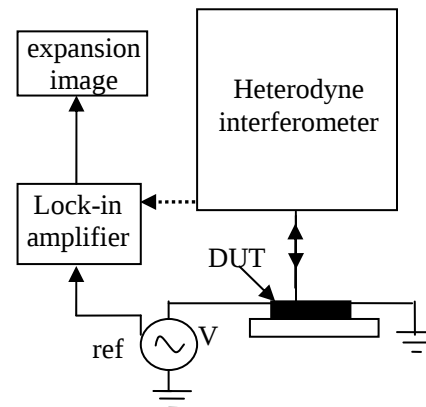
Fig. 6. Interferometer set-up
