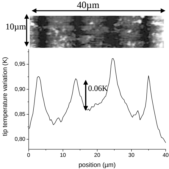
Fig. 10. SThM thermal image and mean temperature variation section signal, f=1 kHz (sample A).
