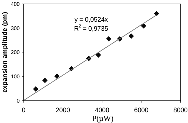
Fig. 4. SJEM expansion amplitude as a function of the power dissipated in each resistor (sample B).
