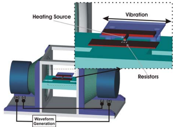
Fig 6. The experimental setup employed for the study of the sensor's dynamic behavior.
