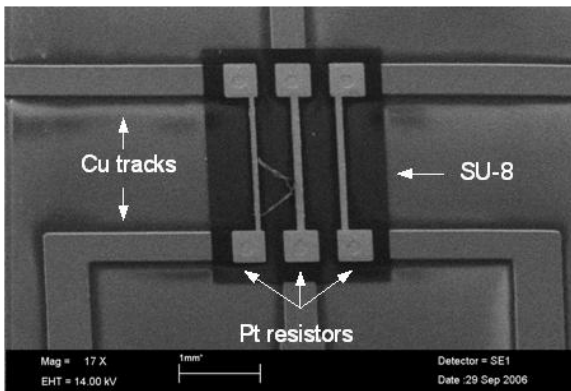
Fig. 2: SEM of the final device. Platinum resistors are in contact with the underlying copper tracks through holes in the SU-8 layer (the latter appears as a dark rectangle)
