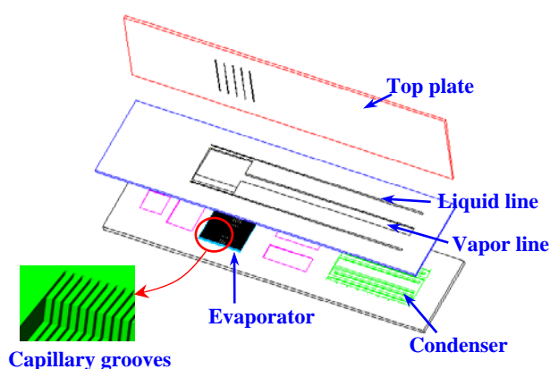
Fig.1 The structure of the micro CPL
