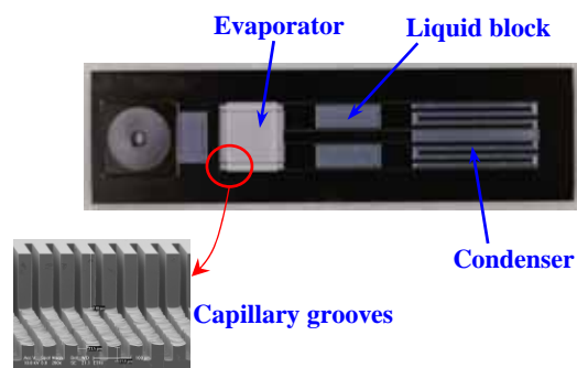
Fig.3 The fabricated micro CPL
