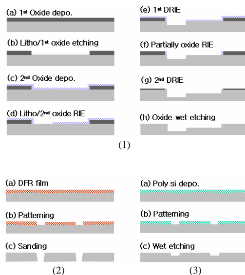
Fig.2 The fabrication process of the micro CPL
