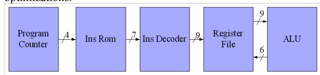
Figure 3. WISP-0 Block Diagram
