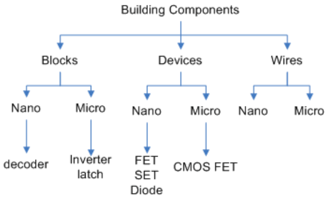
Figure 2. Building components used in architectural model
