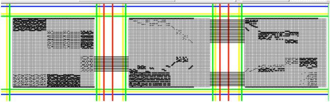
Figure 6. Abstract WISP-0 Layout from NanoMadedo
