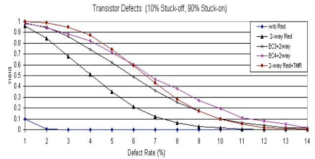
Figure 5. Graph of yield simulator output for WISP-0
