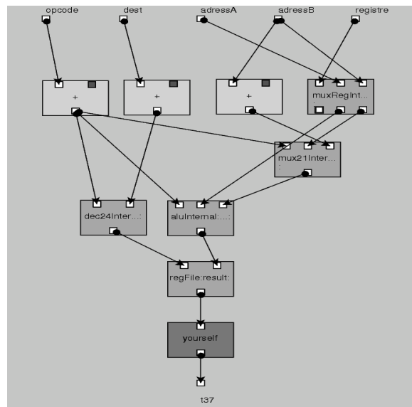
Figure 4. DAG representing ALU and RF
