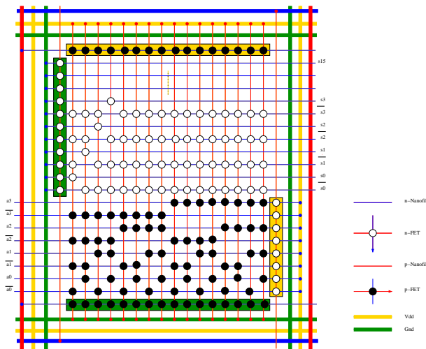
Fig. 4. Address decoder.
