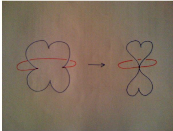
Figure 1: Bifurcation of the conjugate locus (in blue) from an astroid—that is a quatrefoil, as seen from behind—to a double-heart when the initial condition goes to the equator. The same bifurcation occurs on the homotopy regularizing the metric described in [3] when \lambda goes to one. The cut locus (in red) is an open arc for a point on the equator.
