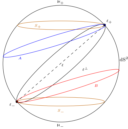
FIGURE 1. In the spherical projective model, A is a horosphere of center l_+ and B is a horosphere of center l_- (drawn with one dimension less than the text).
