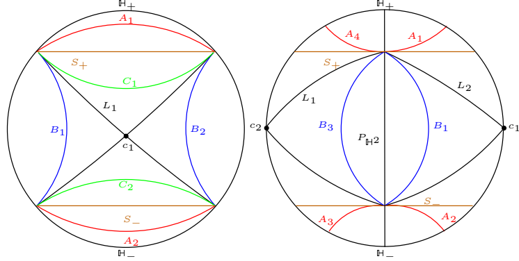
FIGURE 2. In the spherical projective model, A_i are (parts of) hyperbolic caps, B_i are time-like caps, C_i are space-like caps and L_i are light-like caps.
