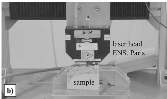
FIG. 4: Measurements of the stylolites surfaces with a laser profilometer. Two different lasers were used. One in Rennes University (a), with a step increment of 125 \mu\text{m} (surface S6) and one at the Ecole Normale Supérieure Paris (b), with increments of 30 \mu\text{m} (surface S10A). (see Table I).
