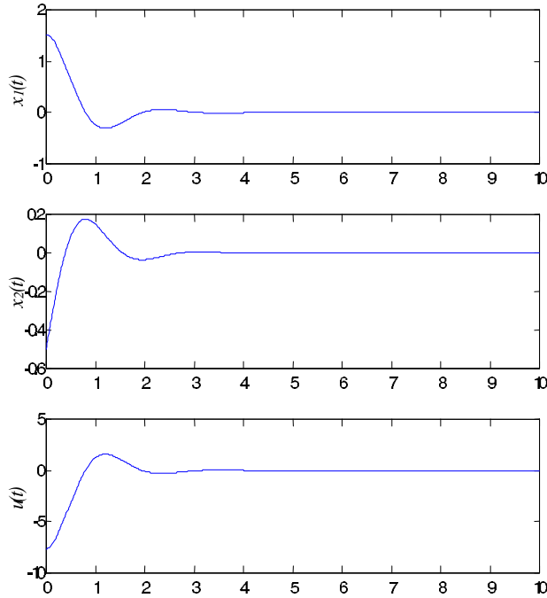
Figure 1. Closed loop system of (40) with x(0) = (1.5 \quad -0.5)
