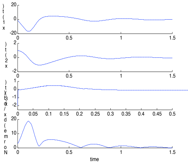
Figure 2: States trajectories with initial values x(0) = [-1 \quad 1 \quad -2]
