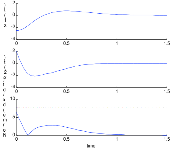
Figure 1: States trajectories of (15) with initial values x(0) = [-2.5 \ 2]
