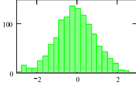
Figure 5. Empirical pdf of the standardized logit's Deltas for French males (1962-1999).
