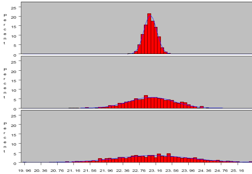
Figure 15. Empirical p.d.f. of residual life expectation at age x = 60 in 20 years (percentiles bar diagram, independent model (top), stochastic logit's Deltas model (middle) and comonotone model (down)).
