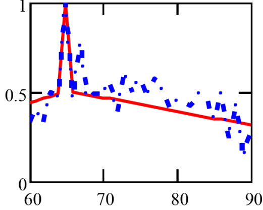
Figure 6. Empirical inter-age correlation coefficients \rho(65, y) for age y (dashed) and smooth fit \tilde{\rho}(65, y) for French males (1969-1999).
