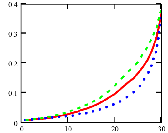
Figure 22. Coefficient of variation of cash-flows of each year (real-life portfolio), independent model (solid), stochastic logit's Deltas model (dashed), comonotone model (dotted).
