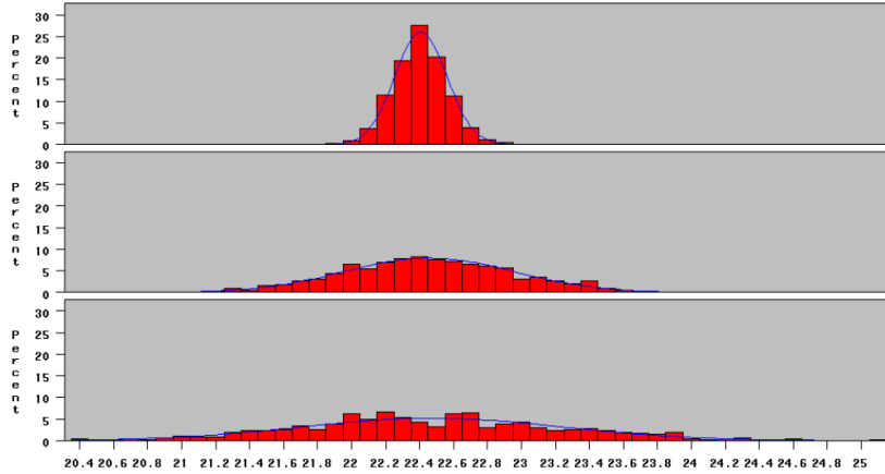
Figure 17. Empirical p.d.f. of prospective residual life expectancy at age x = 60 (percentiles bar diagram, independent model (top), stochastic logit's Deltas model (middle) and comonotone model (down)).
