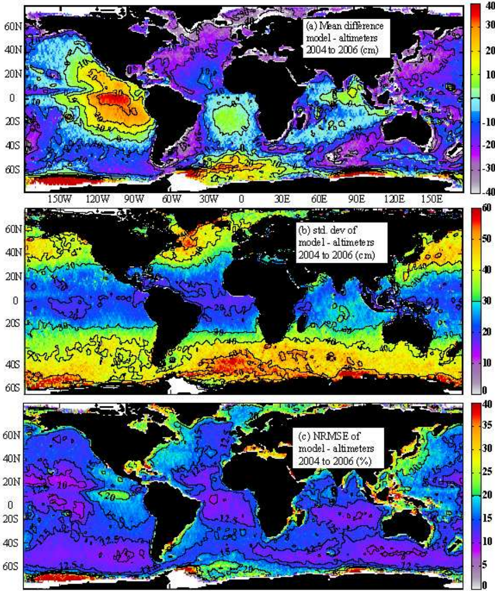
Fig. 2. Statistics for 2004 to 2006, combining data from JASON, ENVISAT and GEOSAT-Follow On (GFO). See Appendix B for satellite data analysis methods.
