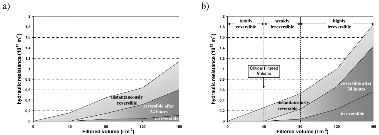
Fig. 4: contribution of resistance according to the filtered volume. a) P=0.6 \text{ bar} – b) P=1.0 \text{ bar} .
