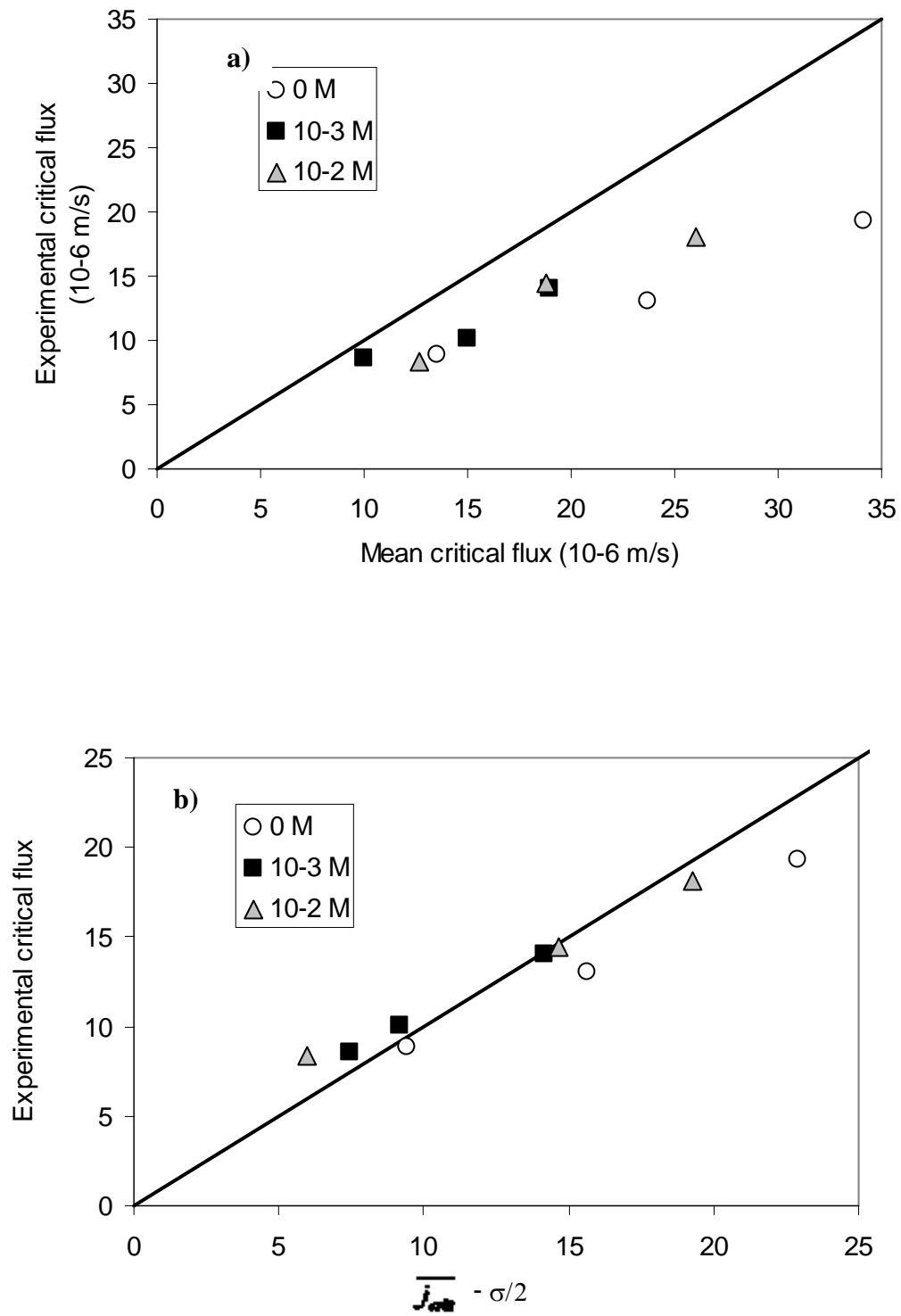
Figure 9. Comparison of the experimental value of critical flux (by a pressure step method [5]) and a) the mean value of critical flux obtained by the modelling or b) the mean value minus half of the standard deviation.
