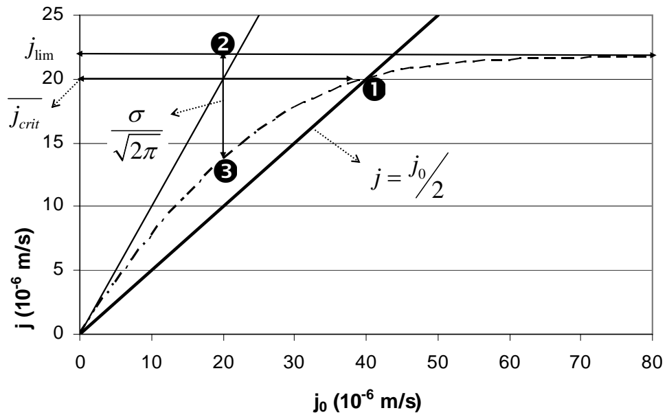
Figure 4. Graphical method to determine parameters of the distribution in critical flux (mean value, \overline{j_{crit}} , and standard deviation, \sigma ) from experimental results (in dashed line) of permeate flux versus water flux.
