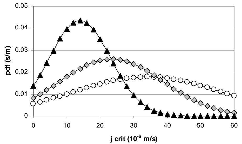
Figure 7. Normal distribution for critical flux used for the fitting of experimental data presented in Fig. 5 and 6 with the DCF model. Mean critical flux and standard deviations are given in Table 2.
