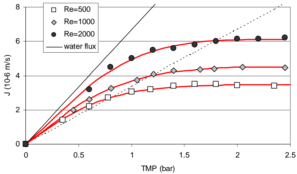
Figure 12. Application of FCFC model to BSA filtration [22]. DCF model (line) allows a very good description of flux- pressure profile (symbols) for various hydrodynamic conditions.
