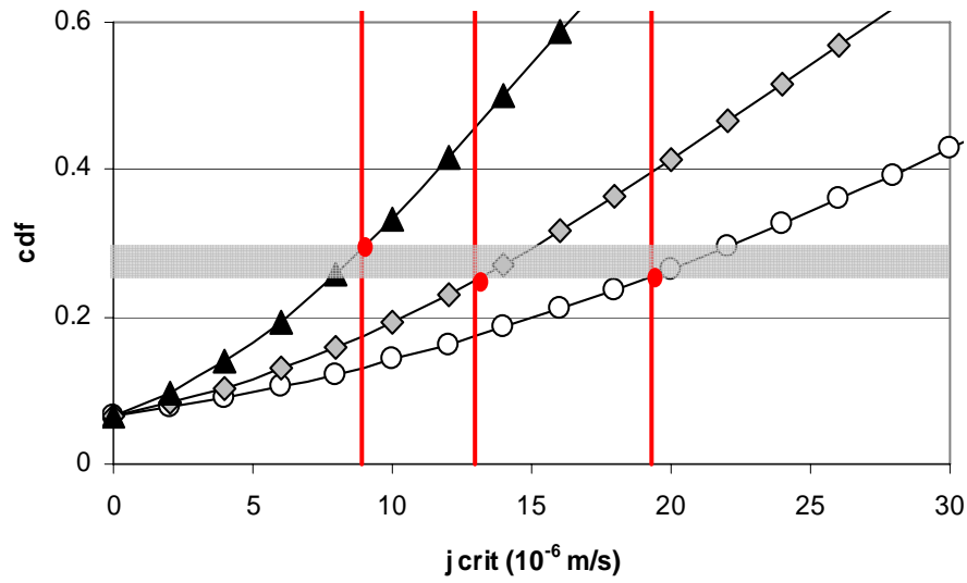
Figure 10. Position of experimental critical flux (vertical lines) with regard to critical flux distribution deduced from DCF model application (Fig. 7). The experimental detection of the critical flux corresponds for this set of experiments to a probability of having reached the critical value of around 0.25-0.3 (field shading).
