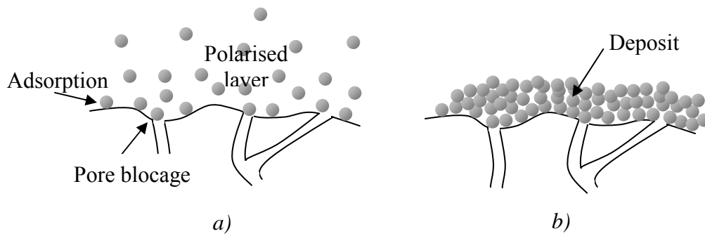
Figure 1. Fouling mechanisms on a membrane a) below critical flux b) above critical flux. Above critical flux, fouling (or more exactly multilayer fouling driven by permeation) becomes predominant.
