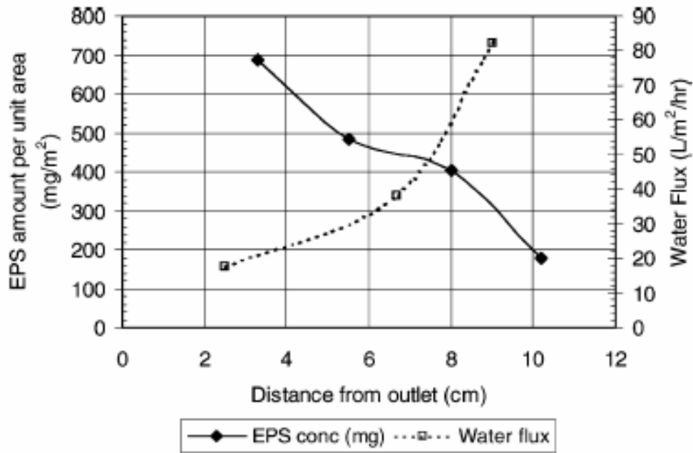
Figure 19. Spatial distribution of extra polymeric substances (EPS) and water flux along a membrane channel (Cho and Fane 2002 [62]). Illustrations of the distribution of a critical flux along the membrane surface.
