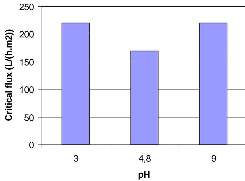
Figure 15. Effect of the pH on the critical flux obtained during flux stepping, experiments using 0,1 wt.% solutions BSA. A minimum is observed near the IEP of BSA [42]
