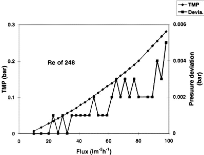
Figure 8. The absolute increase in transmembrane pressure between the two points is plotted as a function of the increasing flux. The total transmembrane pressure is also shown (0.15% BSA, pH 9.7, Re 248). Source Figure 7 of [10]. (It is noted that the original caption in [10] has an error, there should not have been a cross-reference to another Figure.)
