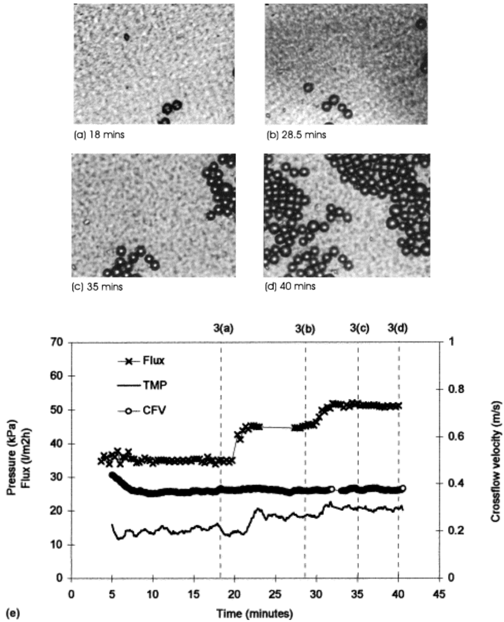
Figure 12. Particle deposition images ((a)-(d)) and the flux and cross-flow conditions (e) in filtration of 11.9 \mu\text{m} latex particles. The time when the images were taken is denoted by the vertical broken lines in (e). [24]
