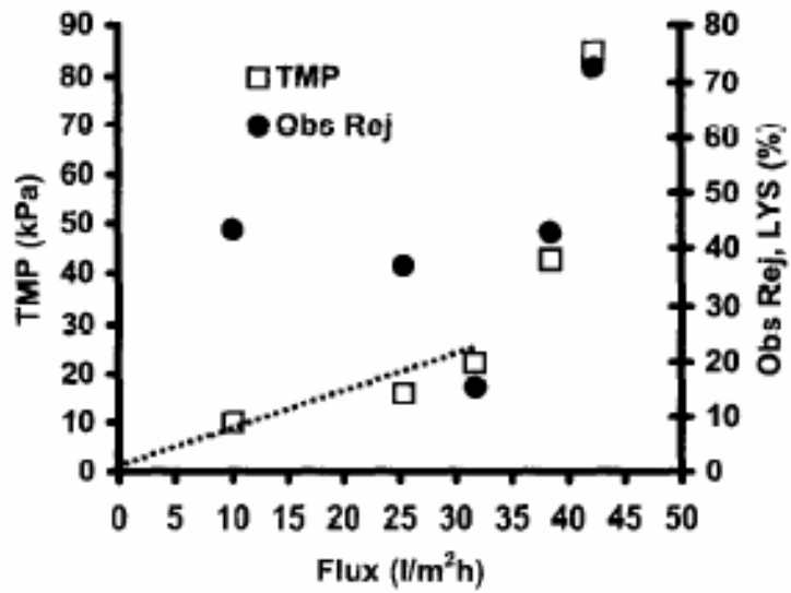
Figure 20. Filtration of a binary mixture of proteins. A minimum of observed rejection in the smaller protein is observed when critical flux is reached [41].
