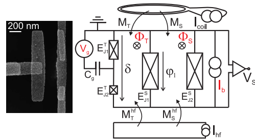
FIG. 1: Electrical schematic of the coupled circuit. The working point is controlled by a dc gate voltage V_g , a current biased I_b and the fluxes \Phi_T and \Phi_S . The current I_{coil} and I_{hf} produces a flux on the SQUID and transistor through respectively the mutual M_S , M_T and M_S^{hf} , M_T^{hf} . The high frequency (hf) line is also used to produce a \mu w flux pulse and a nanosecond flux pulse for the escape measurement of the SQUID. On the left side a SEM image of the asymmetric Cooper pair transistor.
